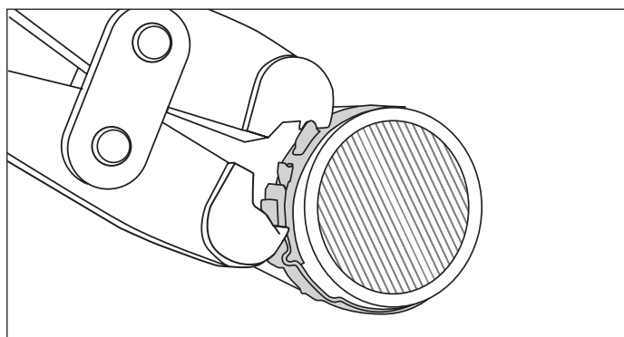
1. Position jaw over tensioning hook.
