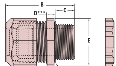
SEALING NUT INTEGRAL SEALING RING
